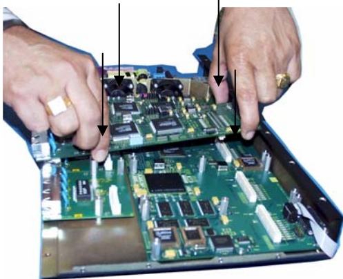
Fig. 3.6.2e Magnum 6KPM daughter board aligned with the bottom female connector for the installation
